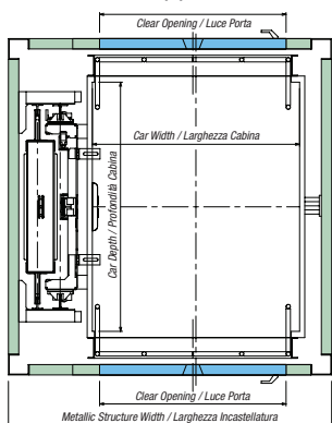
Double entrances opposed Due accessi opposti
