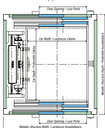
Double entrances opposed Due accessi opposti
