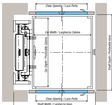
Double entrances opposed Due accessi opposti
